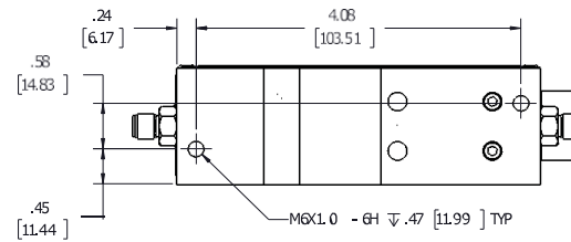
Figure 3 Dimensional Drawing QMC Bottom View
